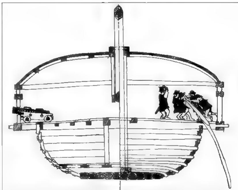
Cross-section of turtle ship with crewmen. The yuloh style of oar is clearly illustrated, and a 'heaven' cannon is rolled out for action.
